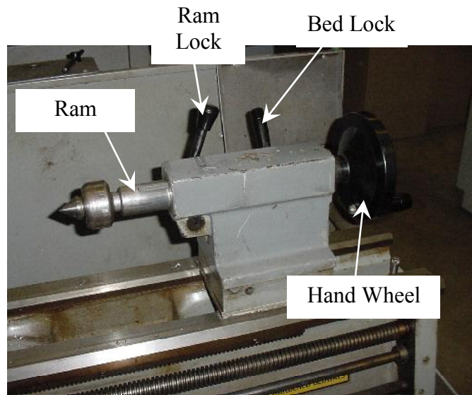
Tail Stock
