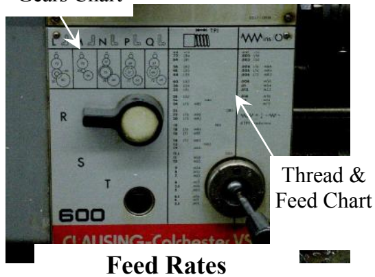
Feed Change Gears Chart
